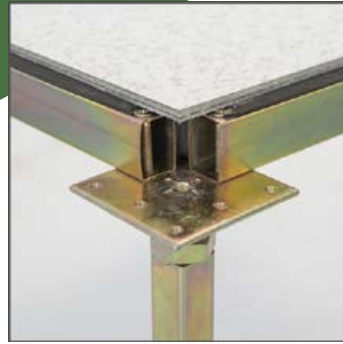
FS SYSTEM BOLT-ON STRINGER SYSTEM
