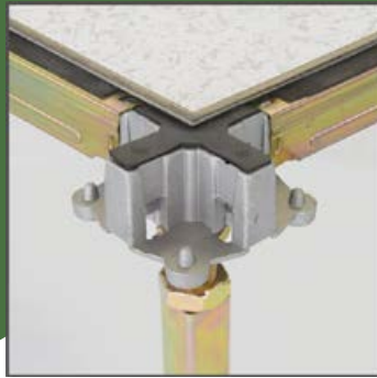
FS SYSTEM SNAP-ON STRINGER SYSTEM
